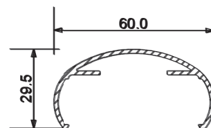
● MAIN COURANTE GC4002
